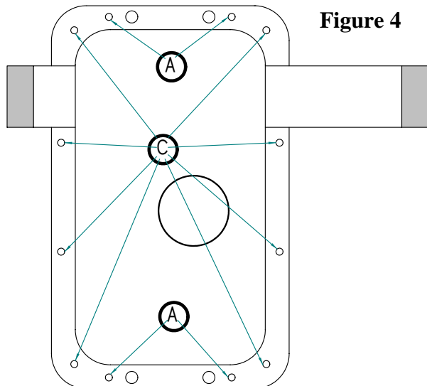
20m Element Housing Installation
